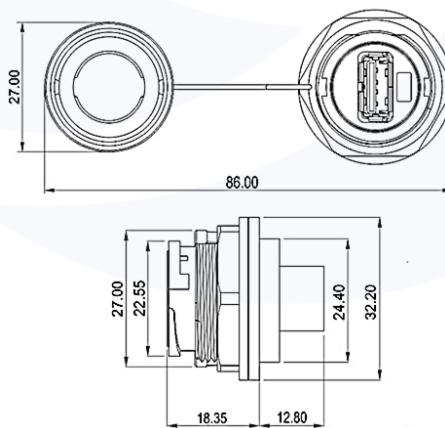
Socket Dimensions figure
